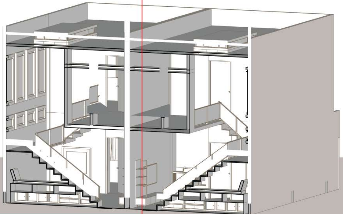
TWIN DUPLEX Diagram: Isometric Section
