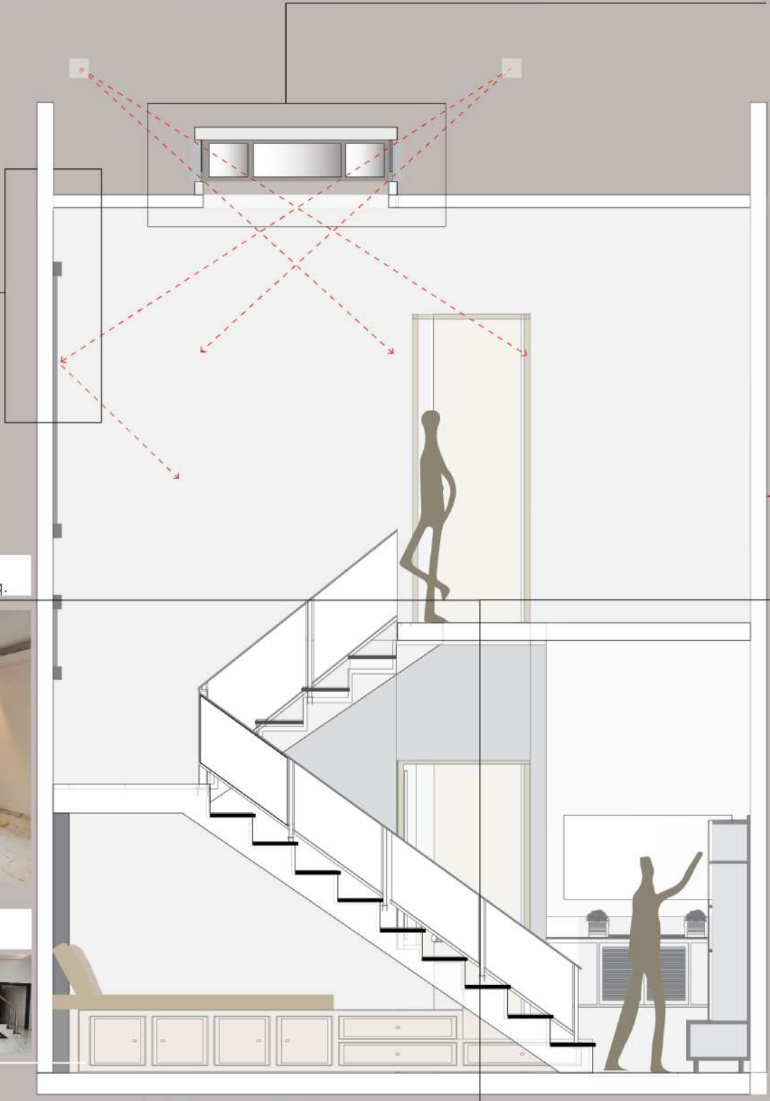
Diagram :Single duplex zoom in Section
