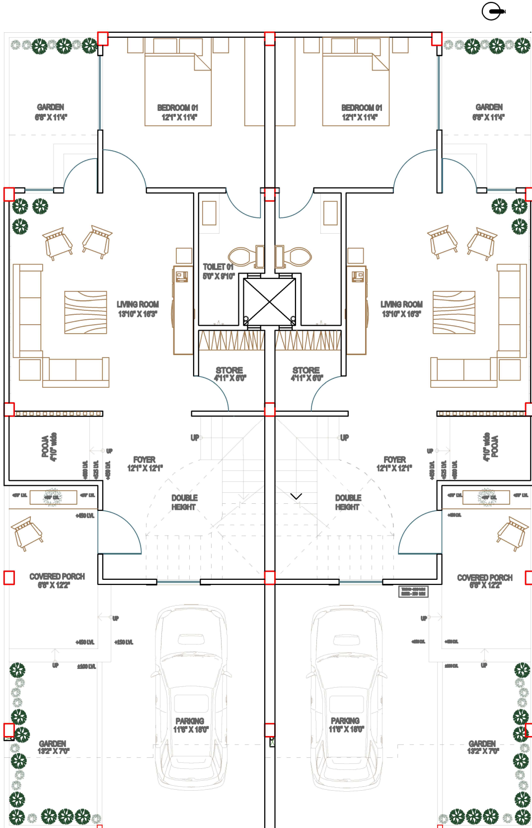
GROUND FLOOR LAYOUT
