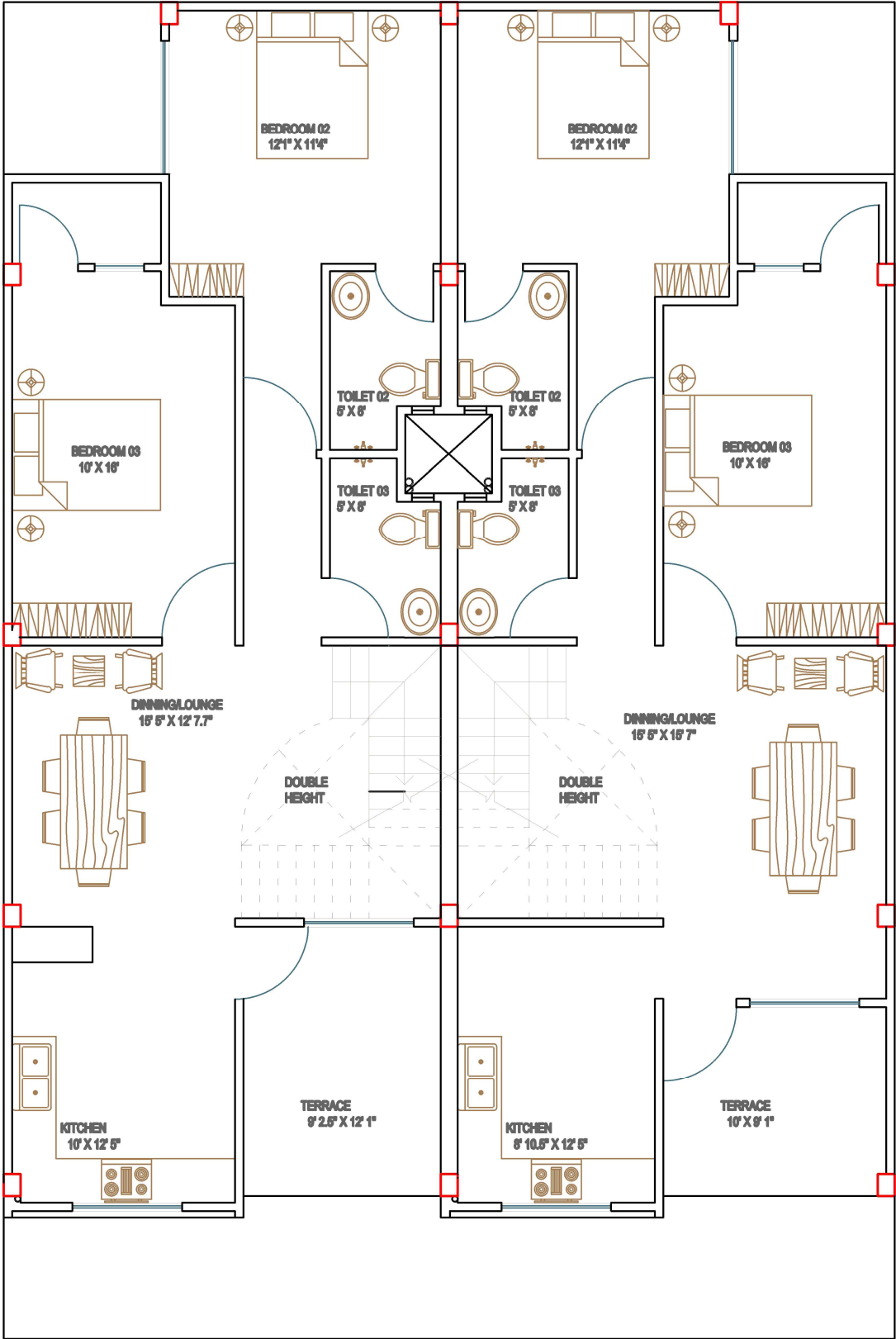
1ST FLOOR LAYOUT
